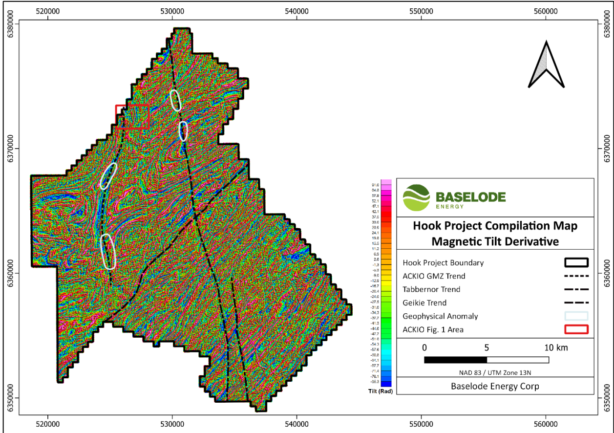
FIGURE 2: Hook project exploration targets (airborne magnetic tilt derivative as background)
