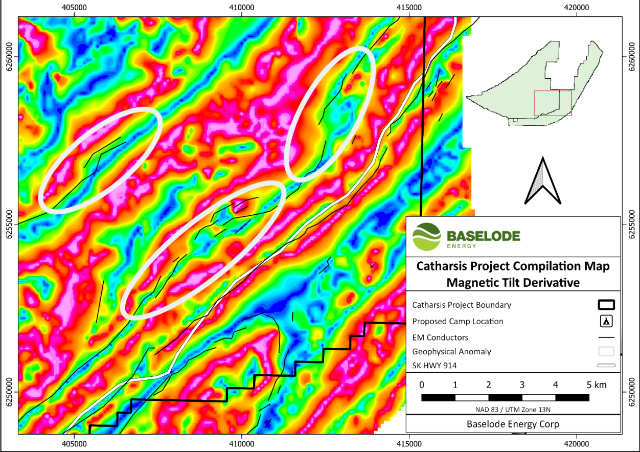
FIGURE 3: Catharsis project exploration targets (airborne magnetic tilt derivative as background)
