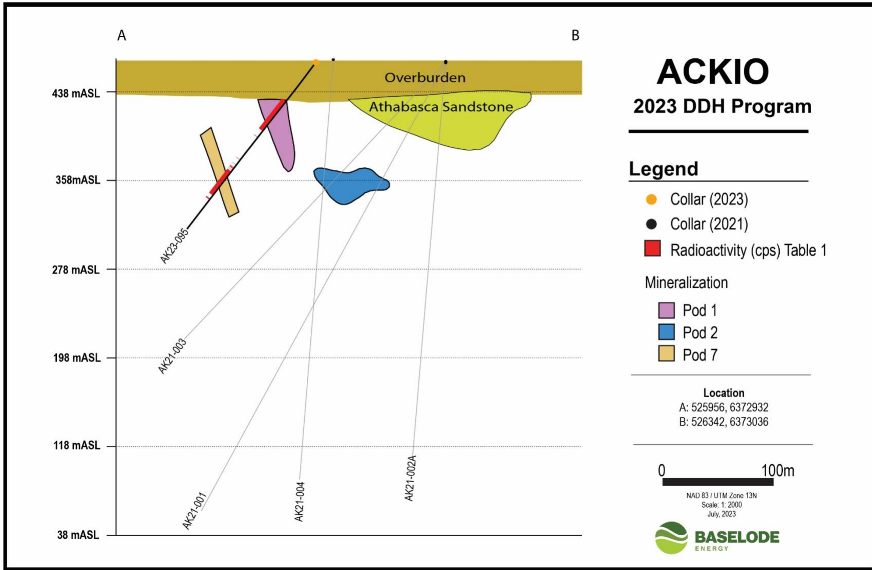
FIGURE 2 – Cross-Section with Drill Hole AK23-095
