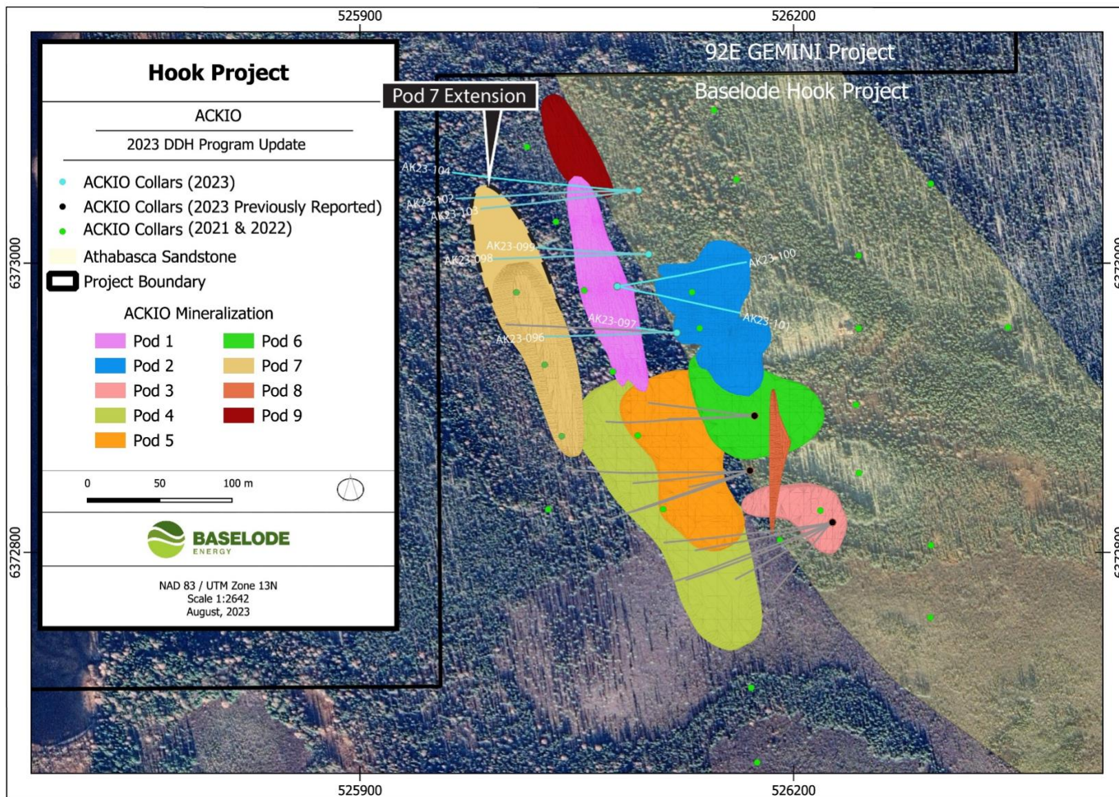
FIGURE 1 – Surface projections of modeled ACKIO uranium mineralization
