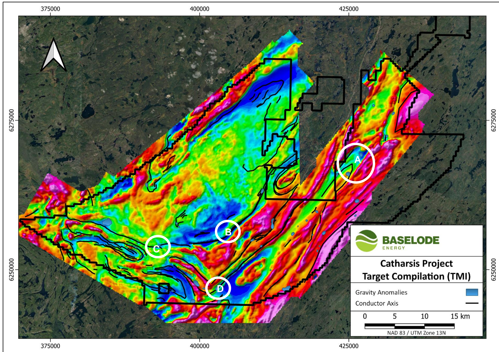
FIGURE 2 – Catharsis project and 2024 diamond drilling target areas A to D (white circles)
