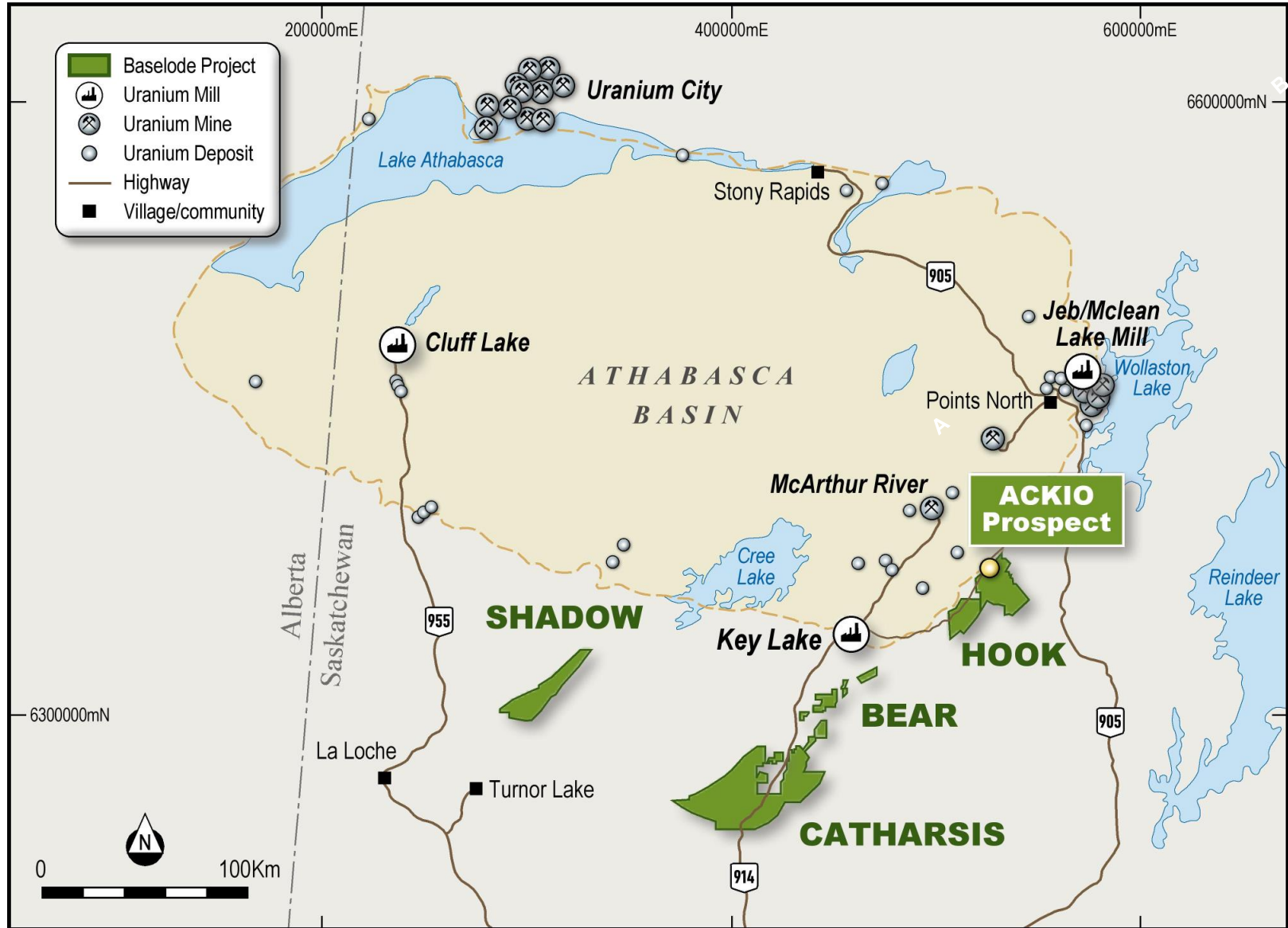
FIGURE 1 – Bear, Catharsis, Hook & Shadow projects location map. ACKIO uranium prospect identified by yellow circle
