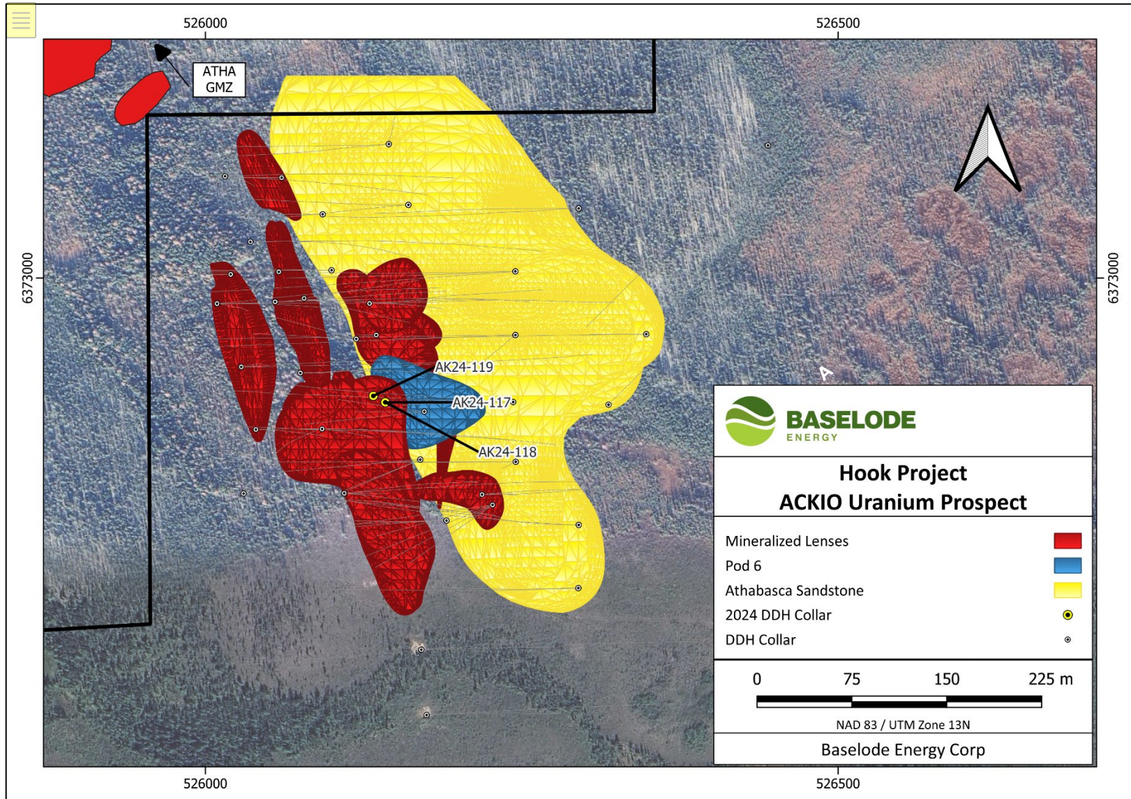
FIGURE 2 – ACKIO Drill Hole Locations
